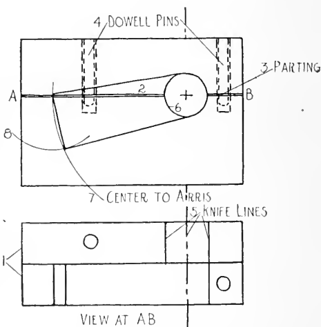
FIG. 545. STOP-OFF CORE-BOX DETAIL.
